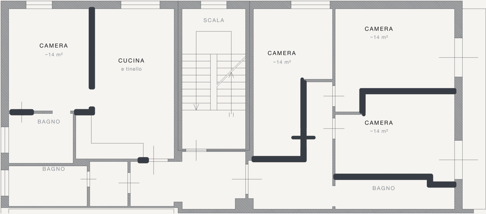
PIANTA DEL PIANO Floor plan CAMERA Double room BAGNO Bathroom CUCINA E TINELLO Kitchen & dining
